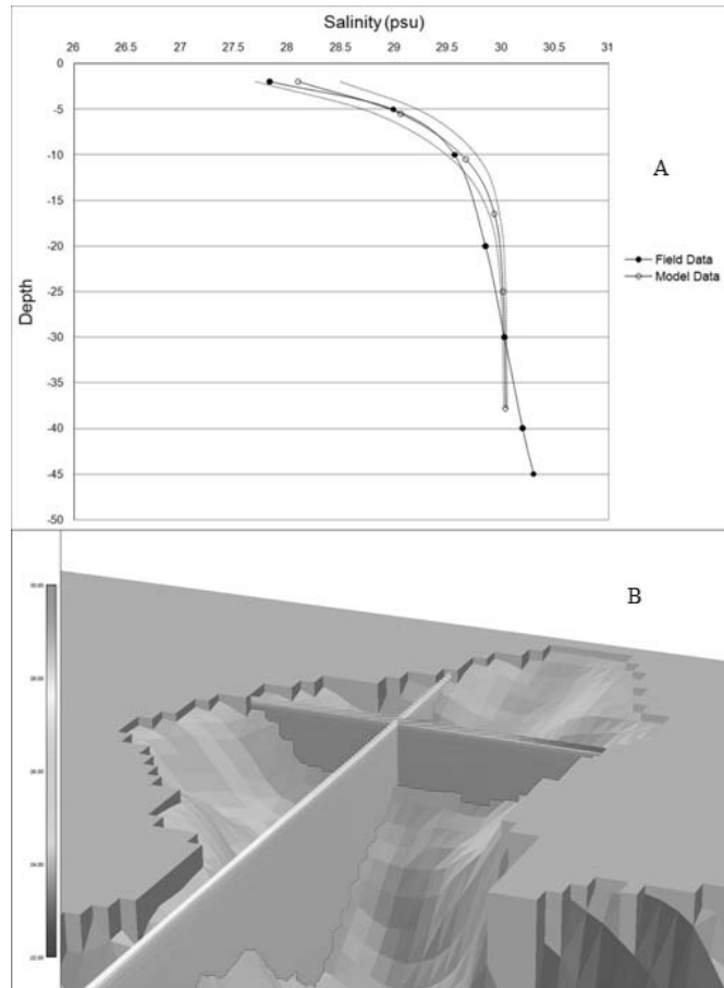
FIGURE 2: Salinity values for model results (○) and available field data (●). The dotted lines represent standard deviation of model results.
